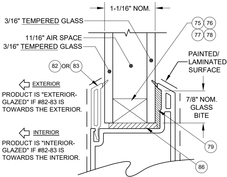
GLASS DETAIL
